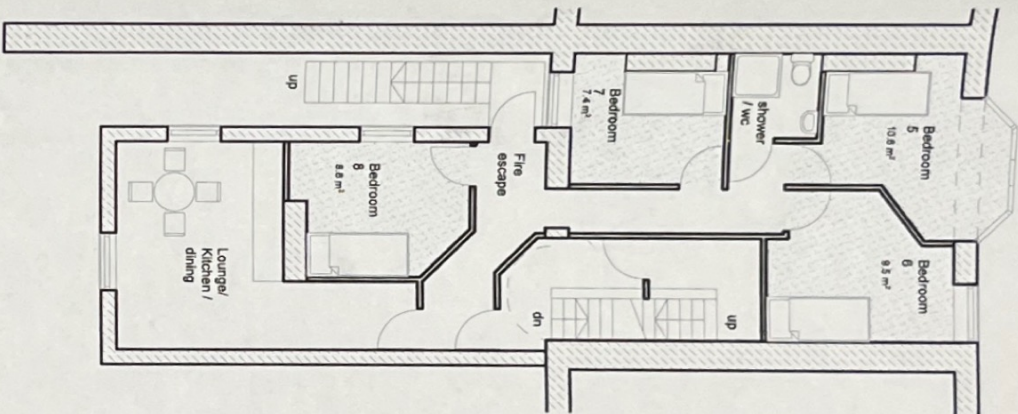
First Floor Layout 1:100
