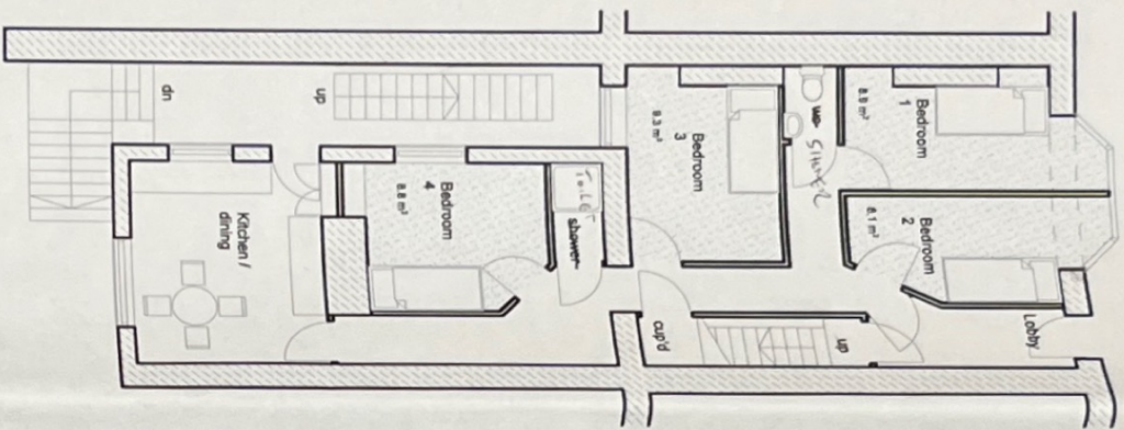
Ground Floor Layout 1:100
